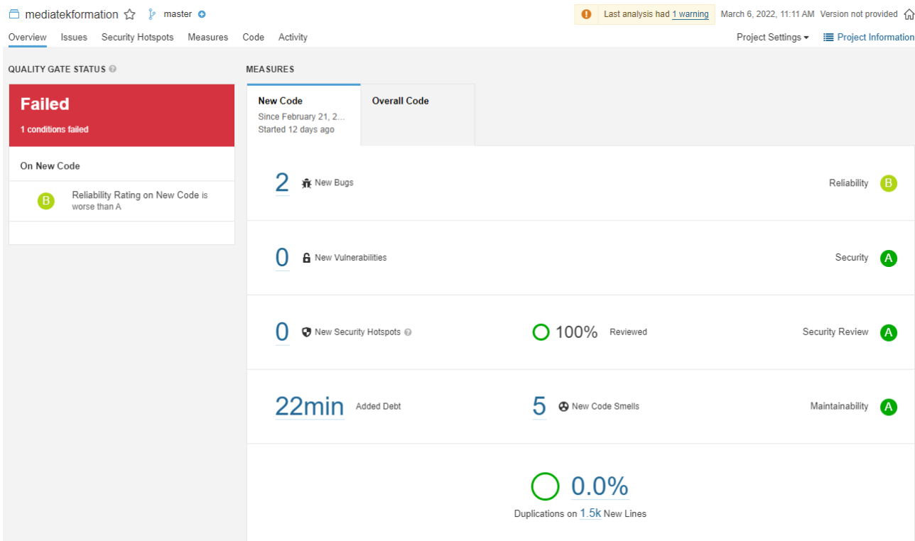
Figure 91: Analyse SonarQube
