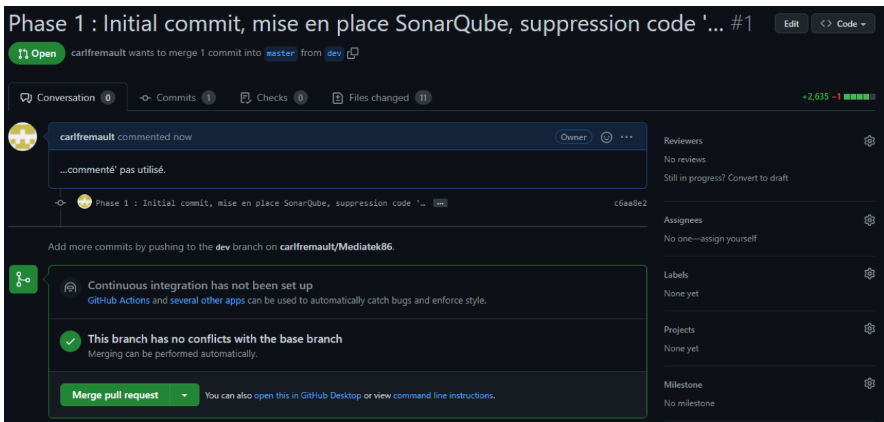
Figure 8: Premier commit
