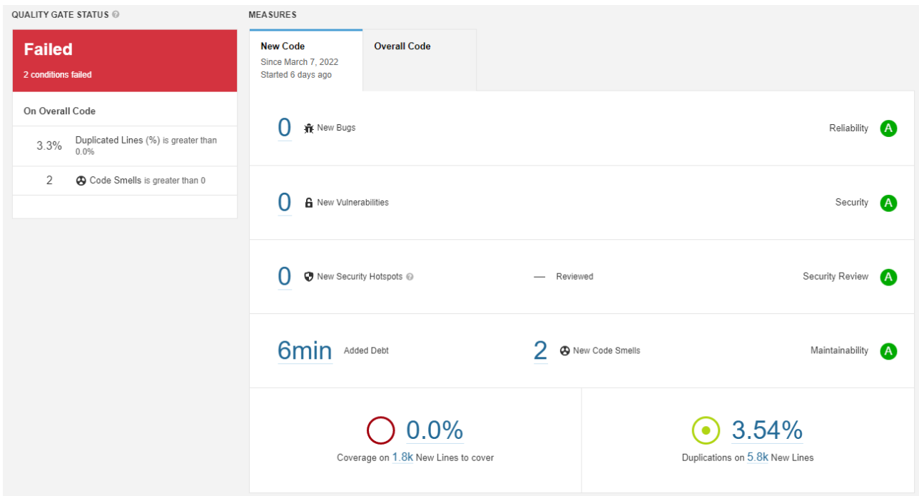
Figure 97: Analyse SonarQube
